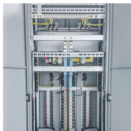
Outdoor Battery Energy Storage (Multi cabinet) - Enetek Power
